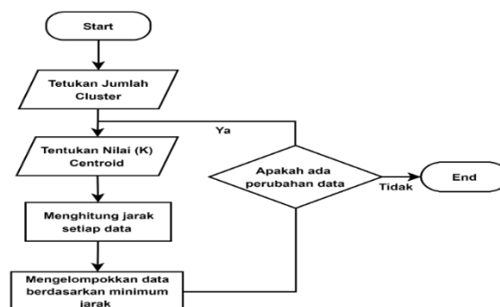
Gambar 1 Flowchart Algoritme K-Means
