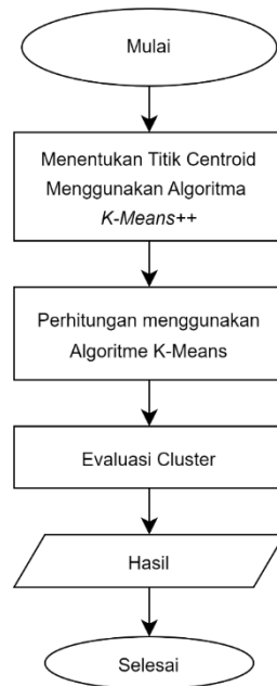
Gambar 2 Tahapan Perhitungan k-Means++
