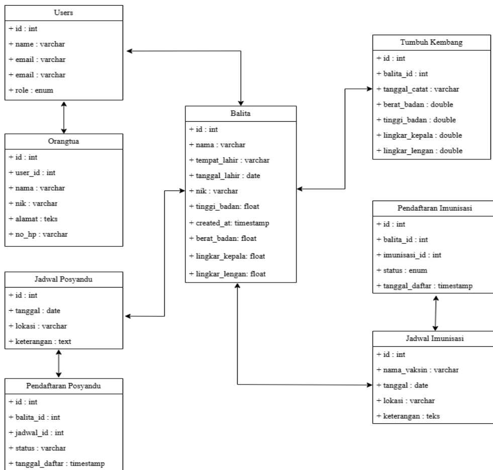
Gambar 4. Class Diagram
